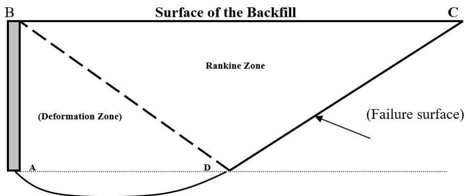
Figure (1): Failure mechanism behind a retaining wall subjected to passive conditions, showing Rankine and deformation zones
