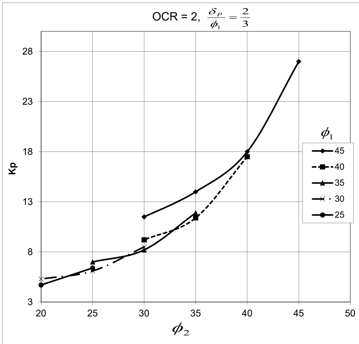
Figure (6): Coefficient of passive earth pressure for OCR = 2, \frac{\delta_p}{\phi_1} = \frac{2}{3}
