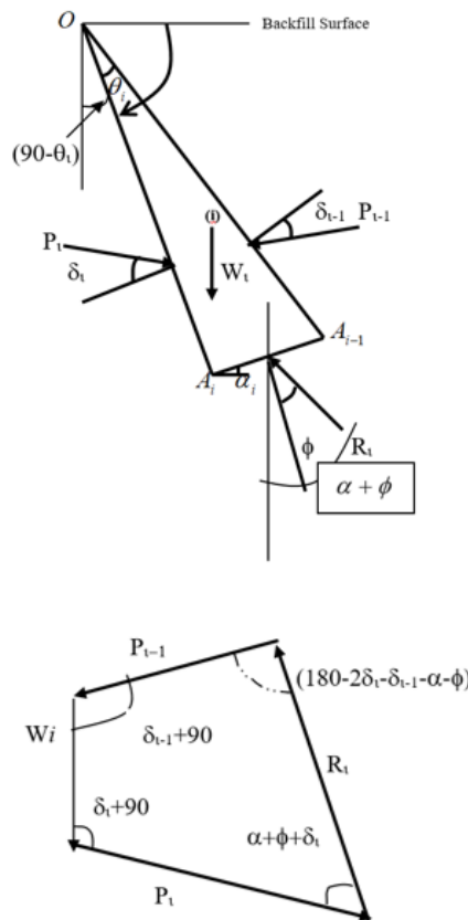
Figure (3): Slice forces' hodograph for a typical slice ( i )
