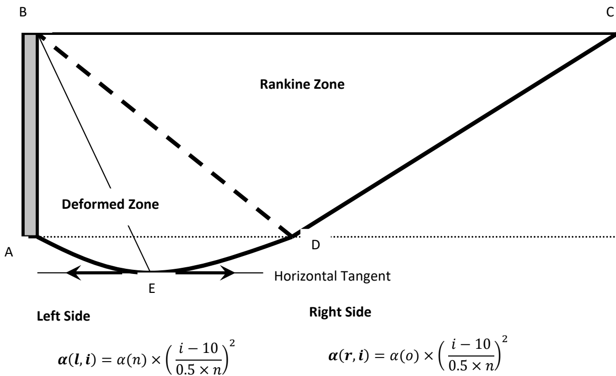
Figure (4): The deformation zone divided into two parts by the horizontal tangent
