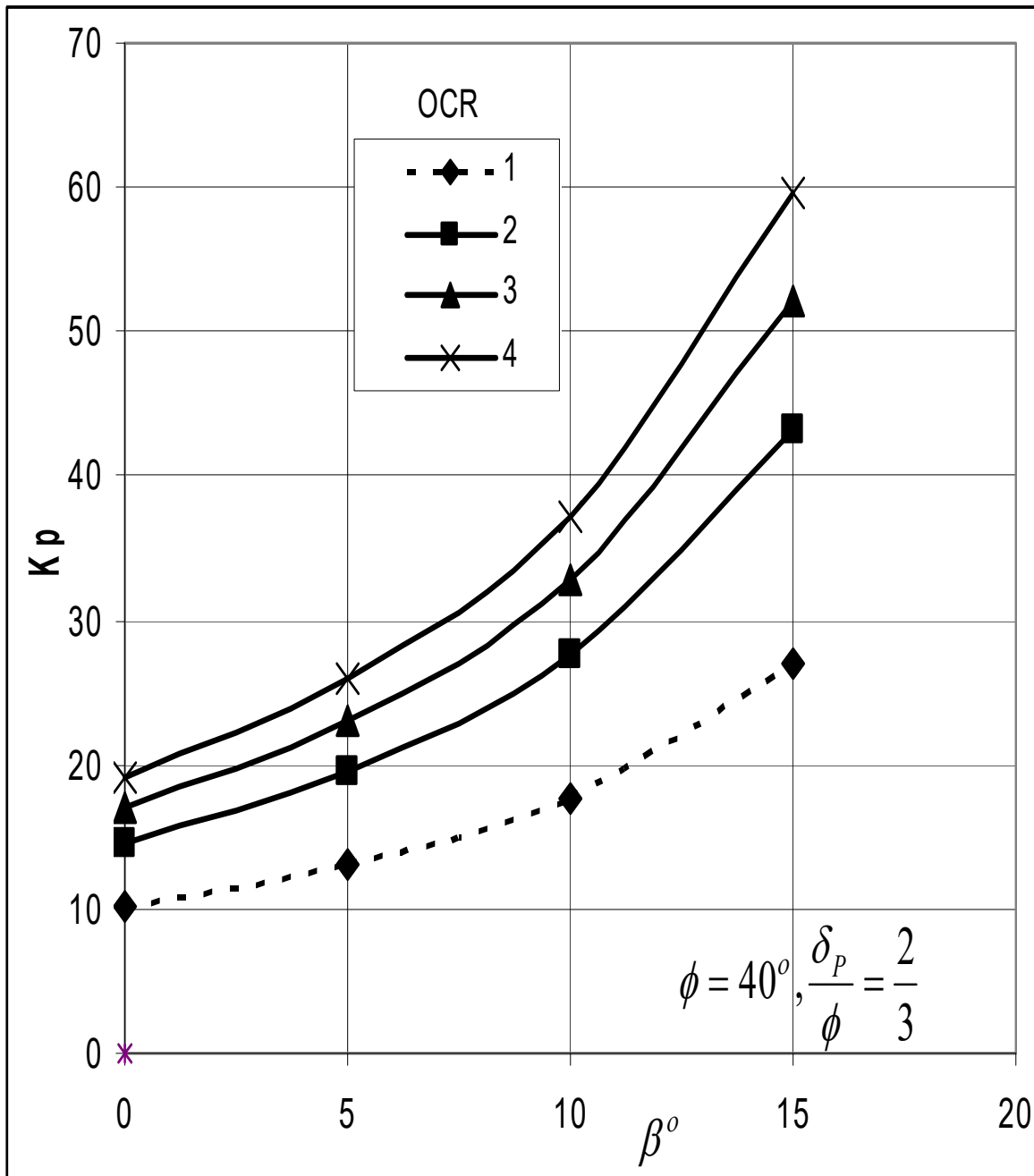
Figure (8): Coefficient of passive earth pressure for inclined homogeneous normally and
