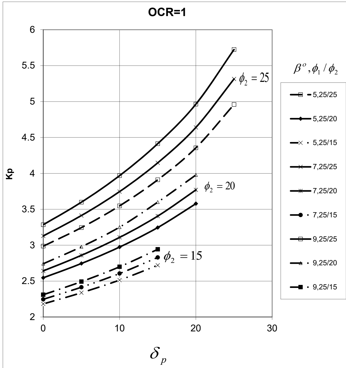
Figure (9): Coefficient of passive earth pressure for inclined backfill for normally consolidated sand
