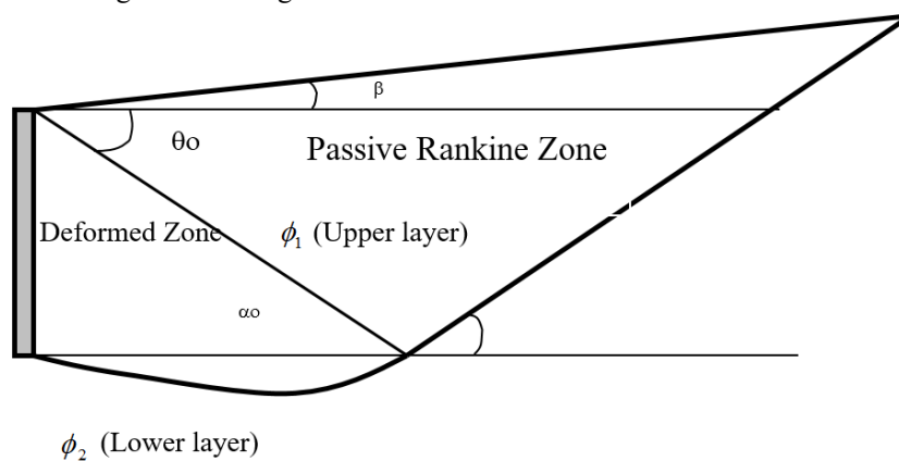
Figure (5): Failure plane for inclined backfill material of an angle behind a retaining wall
