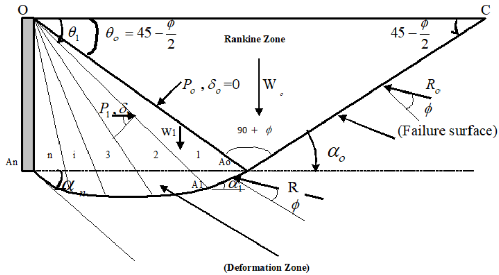
Figure (2): Failure mechanism behind a retaining wall subjected to passive conditions
