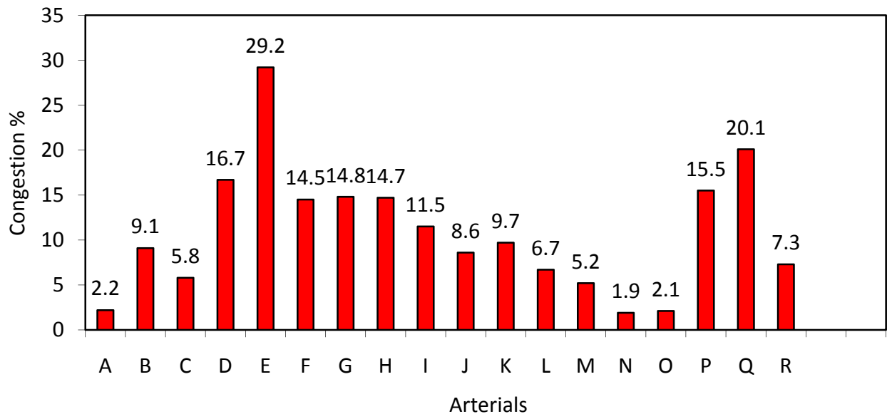
Figure (7): Congestion quantification at peak period
