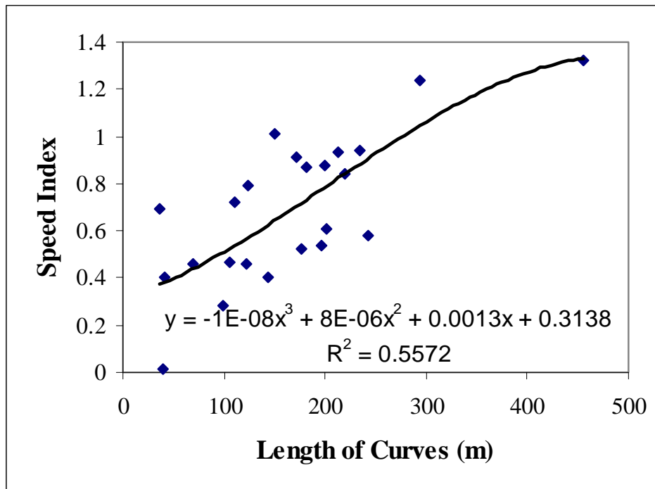
Figure (6): Consistency of horizontal curves according to curvature length
