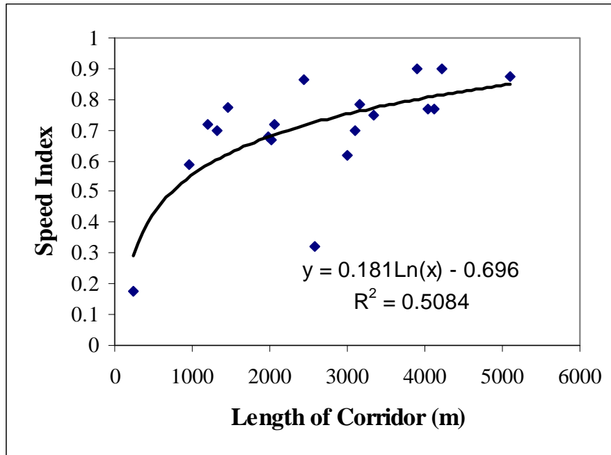
Figure (4): Consistency of segments according to their length
