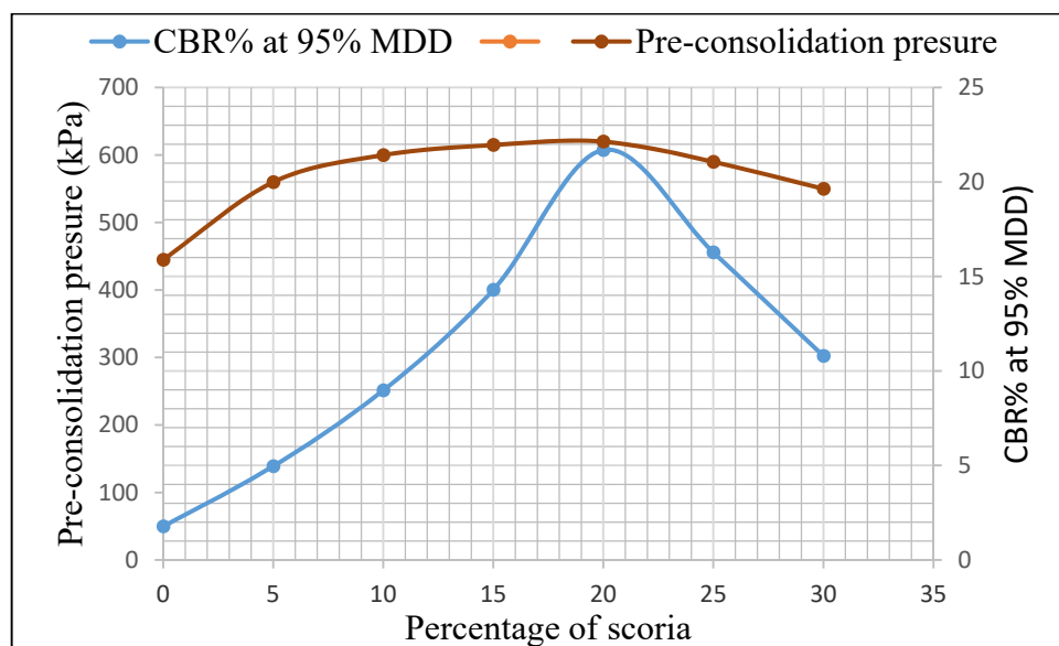
Figure (4): Variation of pre-consolidation pressure and CBR value with different percentages of scoria
