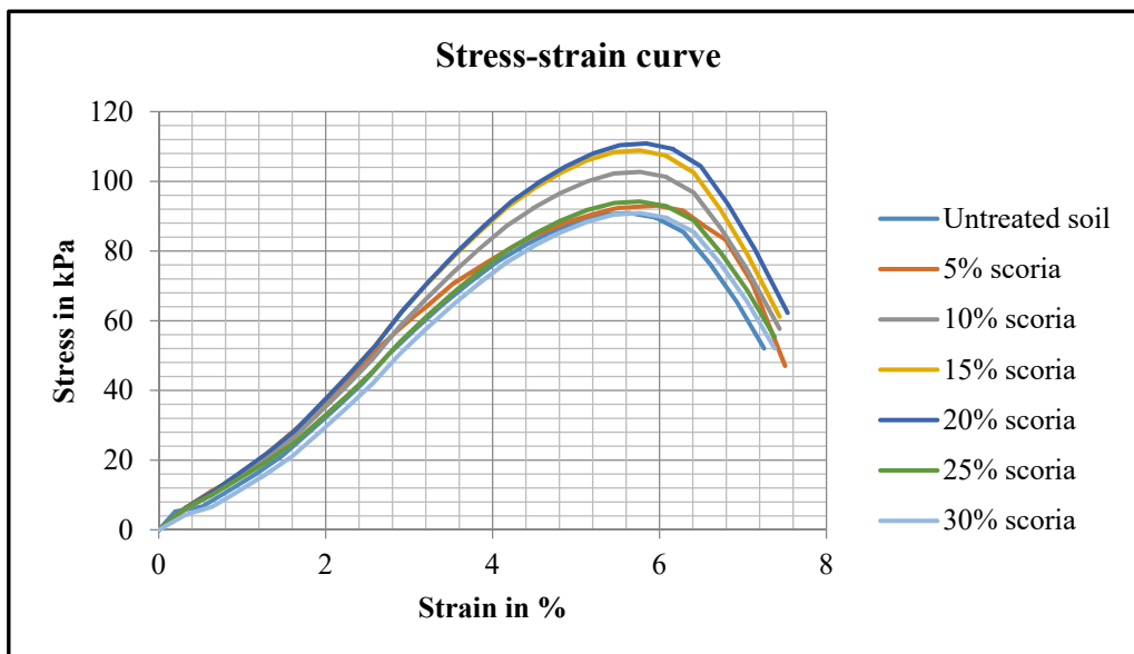
Figure (3): UCS of different % of scoria-treated expansive soil
