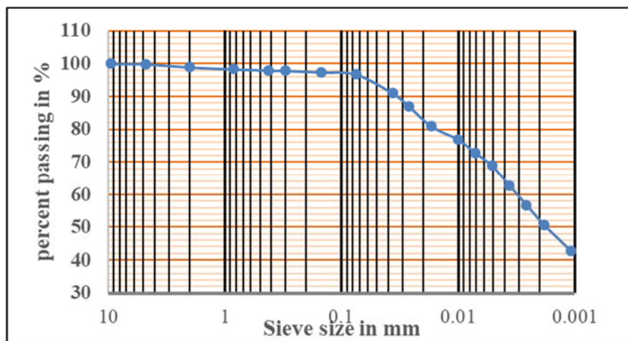
Figure (1): Grain size distribution curve for expansive soil
