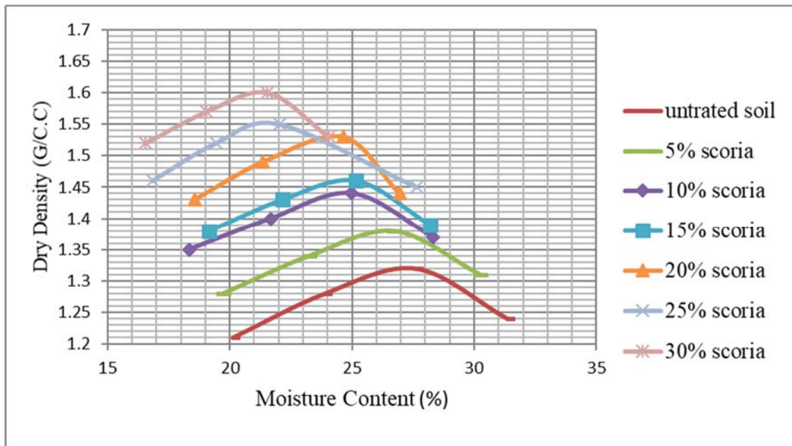
Figure (5): The effect of scoria on the compaction of the soil
