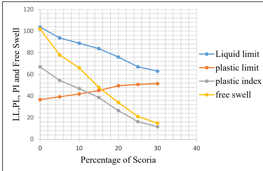
Figure (2): Effect of scoria on swelling potential, liquid limit, plastic limit and plastic index of expansive soil
